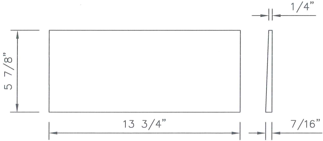
EAVE STARTER
